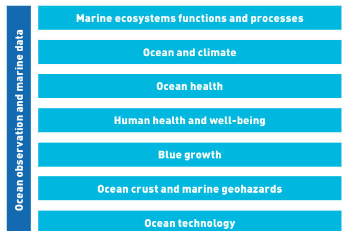
Figure 2.1. Ocean science categories considered in the GOSR.
