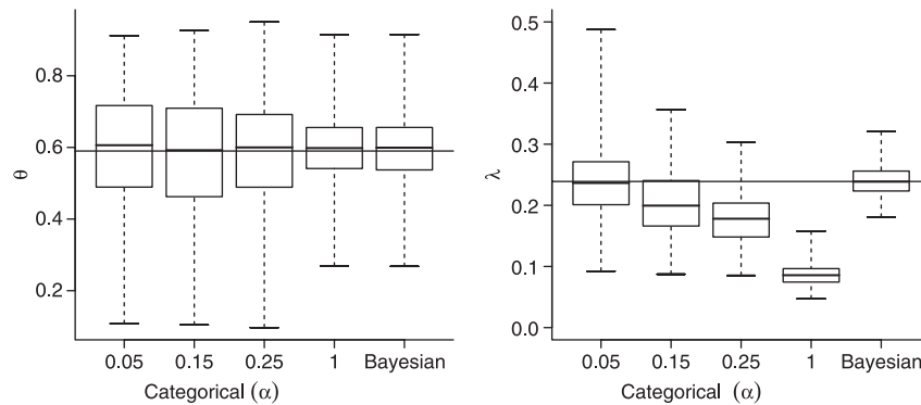
Fig. 2 The distribution of estimates of \theta (the probability that dominant mothers gain maternity over subordinate mothers) and \lambda (the rate at which the chance of paternity drops with distance from an offspring) from the categorical and Bayesian approaches. In the categorical approach, the population-level parameters were estimated from a subset of the offspring that were assigned parents with varying levels of confidence ( \alpha ). It should be remembered that these \alpha values refer to confidence in individual assignments, rather than the population wide confidence usually used. Ninety-five per cent (95%) confidence at the population level corresponds to roughly \alpha = 0.15 in this example. The whiskers of each box represent the minimum and maximum estimates, the boxes represent the interquartile range, and the median of the distribution is represented by the central line. The true underlying values of \lambda and \theta are 0.239 and 0.59, respectively, for each of the 300 simulated test data sets. These values are represented by horizontal lines.
